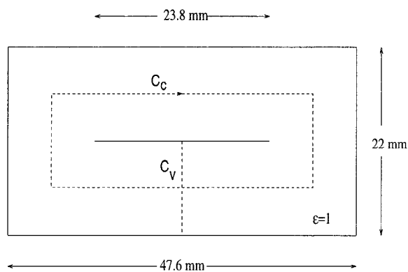
Figure 2: Stripline Geometry.
